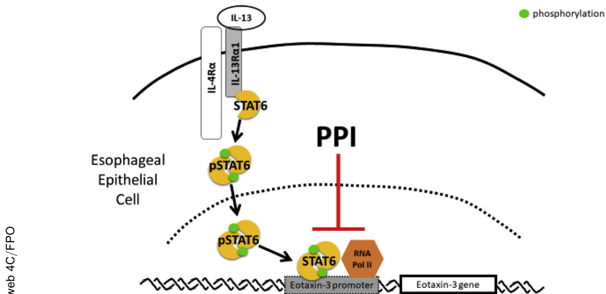
Supplementary Figure 3. Proposed Mechanism of PPI inhibition of Th2-cytokine-stimulated eotaxin-3 expression. Th2 cytokine, IL-13 (or IL-4), can stimulate eotaxin-3 expression via signal transducer and activator of transcription 6 (STAT6) signaling in esophageal epithelial cells. However, in the presence of a PPI such as omeprazole, binding of both STAT6 and RNA polymerase II (RNA Pol II) to the eotaxin-3 promoter is decreased, and transcription of eotaxin-3 mRNA is reduced.
